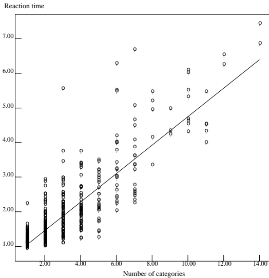
Figure 10: Number of categories in which each token of ALL was found (including the correct answer) vs. reaction time.
